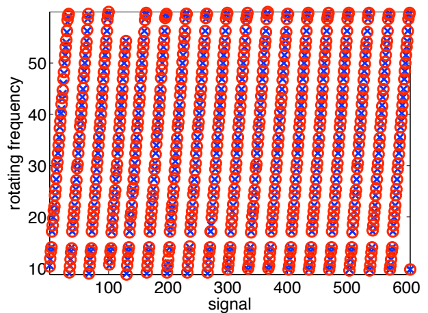
Fig. 4. Comparison between the actual (o) and automatically estimated (x) rotating frequencies.
