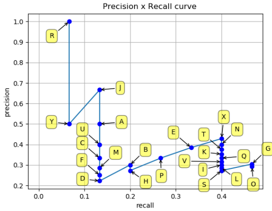
Fig. 4: Precision x Recall curve with values calculated for each detection in Table I.
