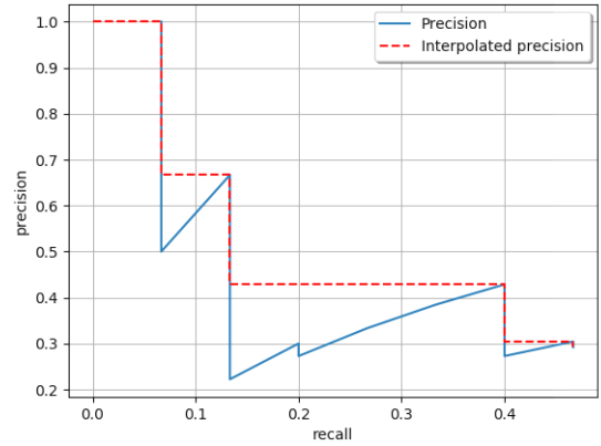
Fig. 6: Precision x Recall curves of points from Table I applying interpolation with all points.
