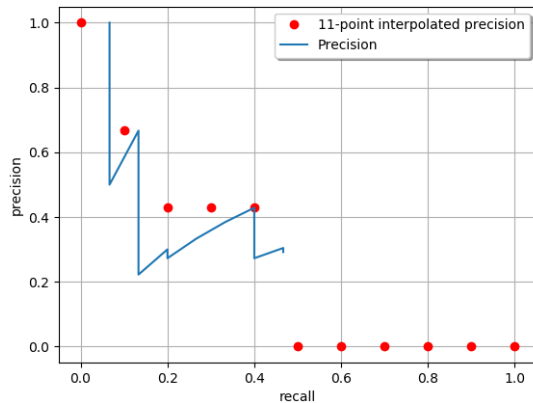
Fig. 5: Precision x Recall curves of points from Table I using the 11-point interpolation approach.
